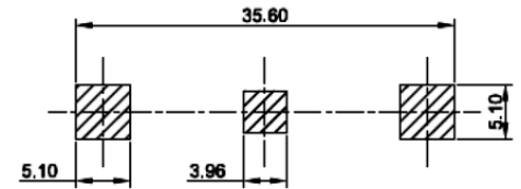
PCB MOUNTING LAYOUT
