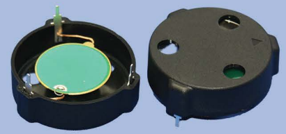
CT51P-30T250-1 Diameter: 51.5 mm Frequency: 2500 Hz
